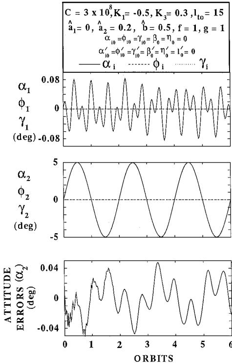
Fig. 4 Typical chase-slewing maneuver response for desired harmonic variations in pitch angle for lower satellite platform.
